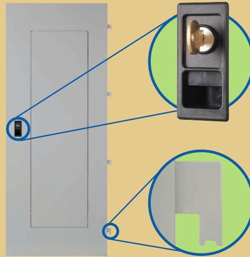
New Lock and Stand-Alone Trim and Bottom Flange Hanger with Notch
